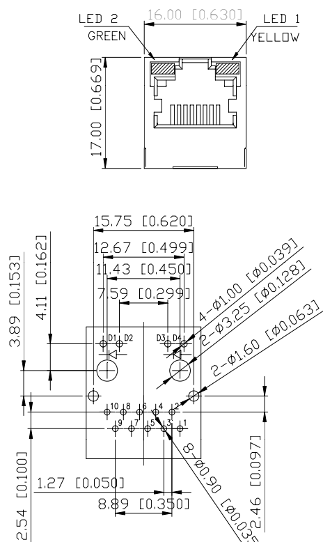
SUGGESTED PCB LAYOUT (TOP VIEW)
